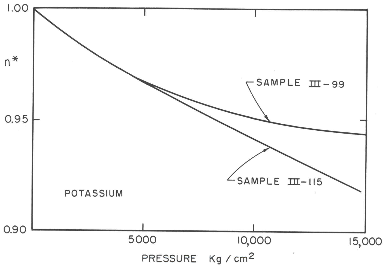
FIG. 3-12 n^* , NORMALIZED. ELECTRONS/ATOM VS. PRESSURE.
